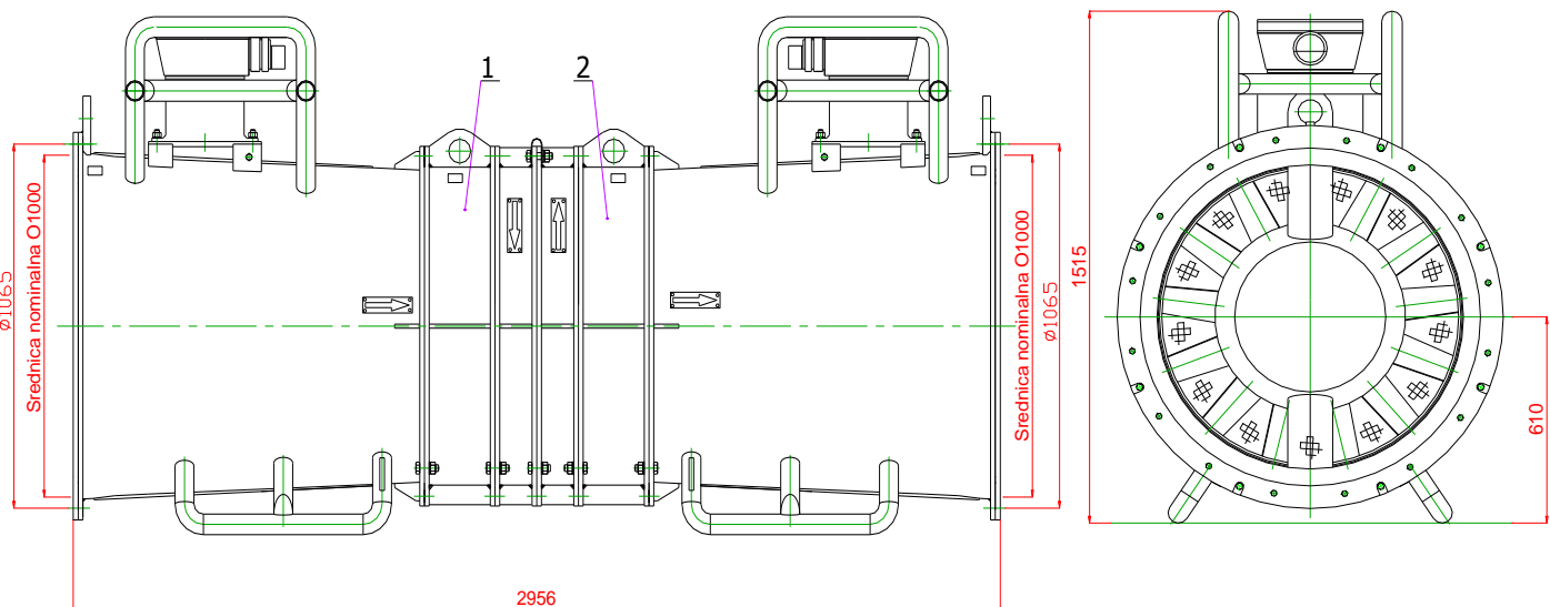
1. Set of inlet I-55/2N/P; 2. Steering I-55/2N/P
